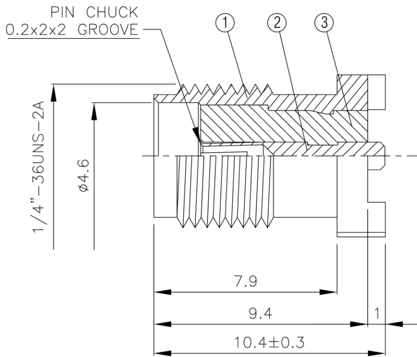
Figure 5-3 RF SMA Connect Drawing
